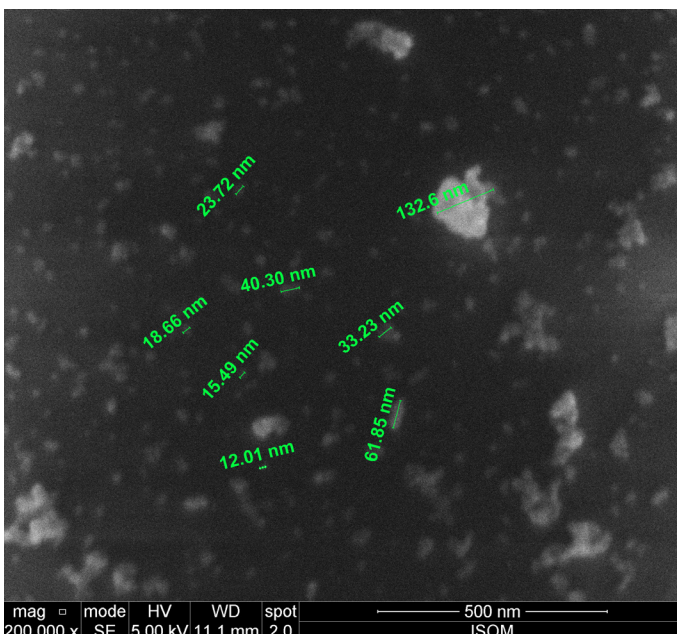
Scanning electron microscopy image of magnetic nanoparticles
